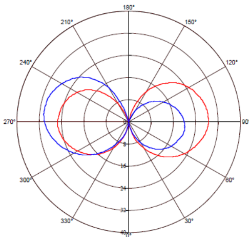
Photometric Diagram
