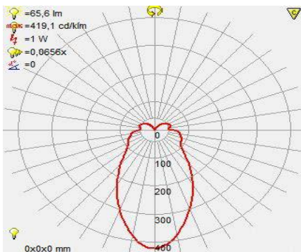
Photometric Diagram
