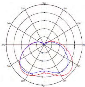
Photometric Diagram
